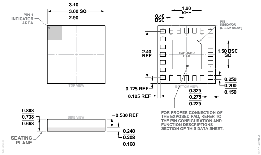
Figure 25. 24-Terminal Land Grid Array [LGA] 3 mm x 3 mm Body and 0.738 mm Package Height (CC-24-12) Dimensions shown in millimeters
