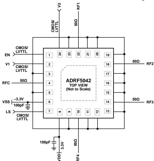
Figure 24. Application Circuit
