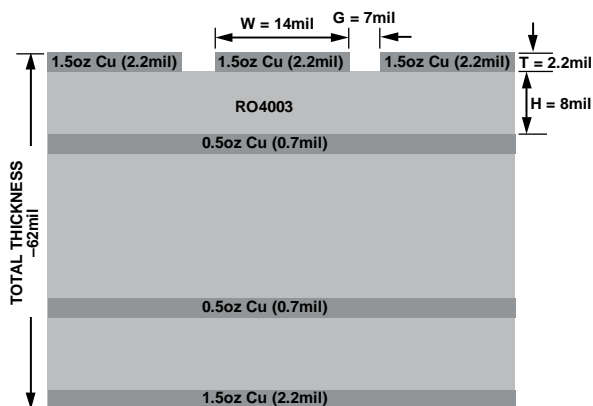
Figure 22. Evaluation Board Stackup, Cross Sectional View
