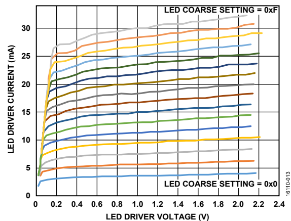
Figure 12. LED Driver Current vs. LED Driver Voltage at 10% Drive Strength, Fine Setting at Default
