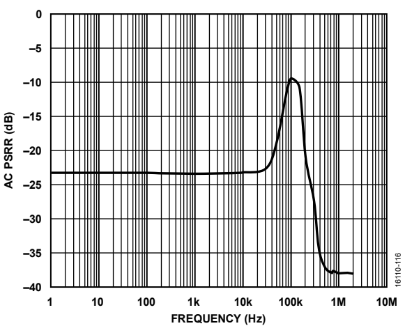
Figure 16. AC PSRR vs. Frequency for 75% Full-Scale Input Signal
