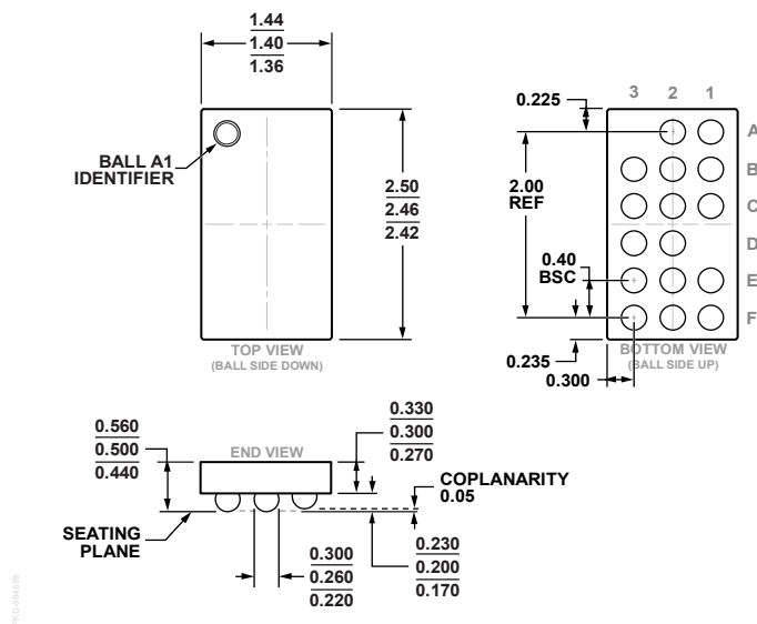
Figure 57. 16-Ball Wafer Level Chip Scale Package [WLCSF] (CB-16-18)
