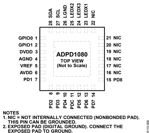
Figure 6. 28-Lead LFCSP Pin Configuration (ADPD1080)
