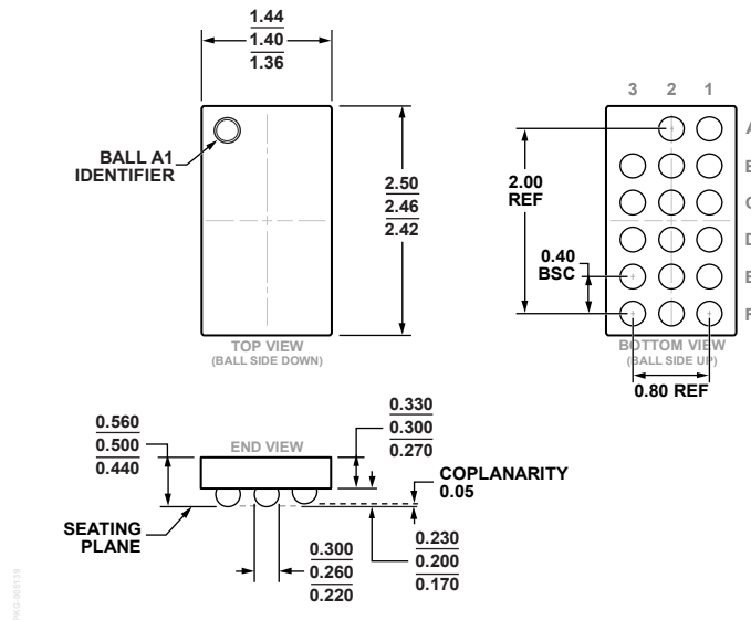
Figure 58. 17-Ball Wafer Level Chip Scale Package [WLCSP] (CB-17-1)
