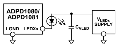
Figure 40. V_{LEDx} Supply Schematic
