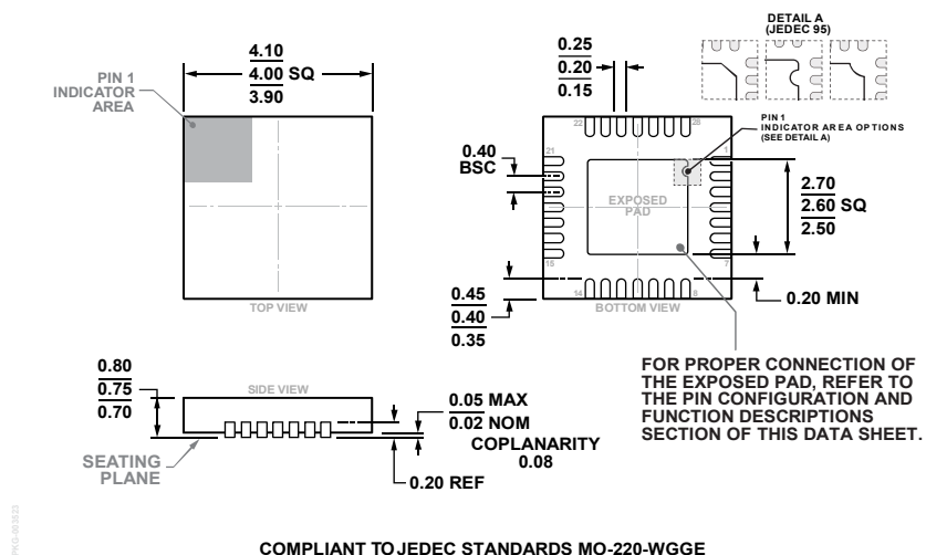
Figure 56. 28-Lead Lead Frame Chip Scale Package [LFCSP] 4 mm × 4 mm Body and 0.75 mm Package Height (CP-28-5)
