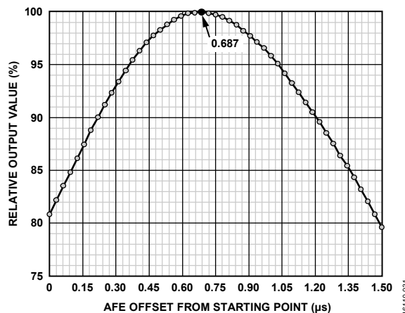
Figure 31. AFE Sweep Example
