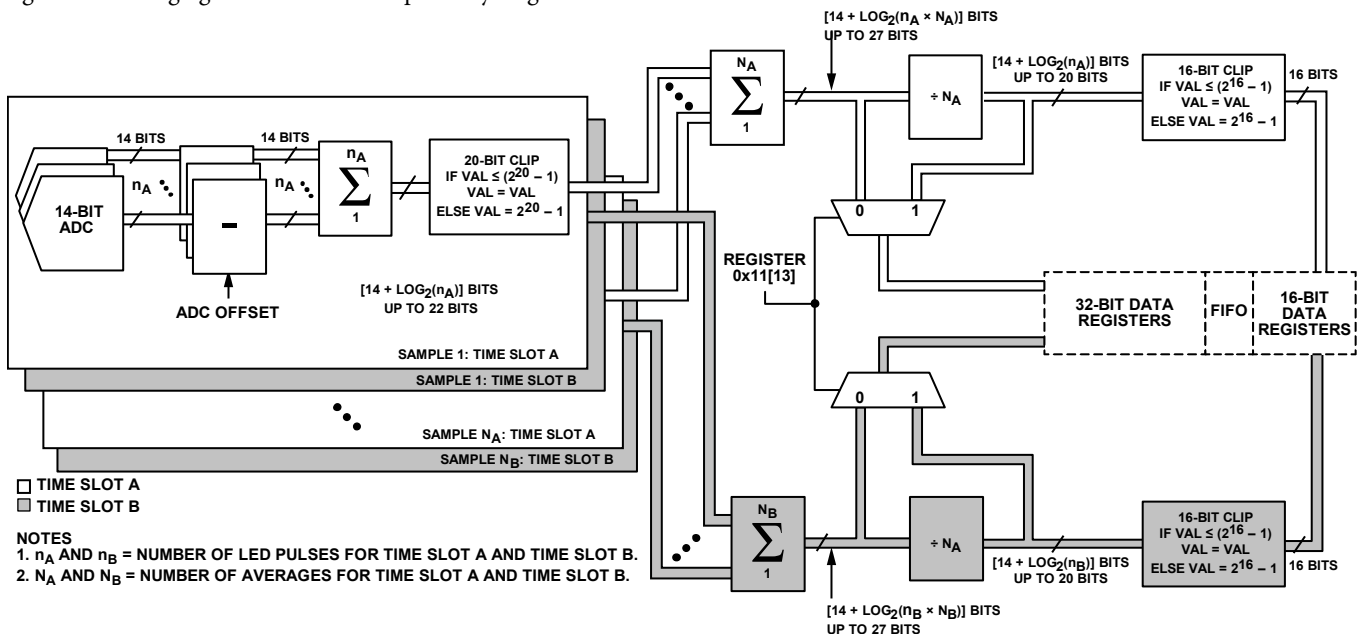
Figure 28. ADPD1080/ADPD1081 Datapath
