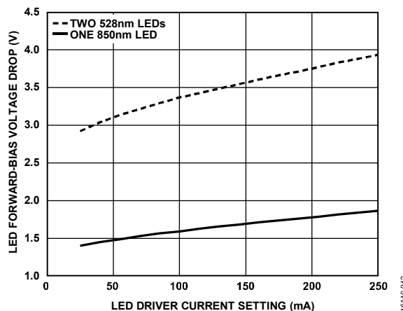
Figure 42. Example of the Average LED Forward-Bias Voltage Drop as a Function of the LED Driver Current Setting
