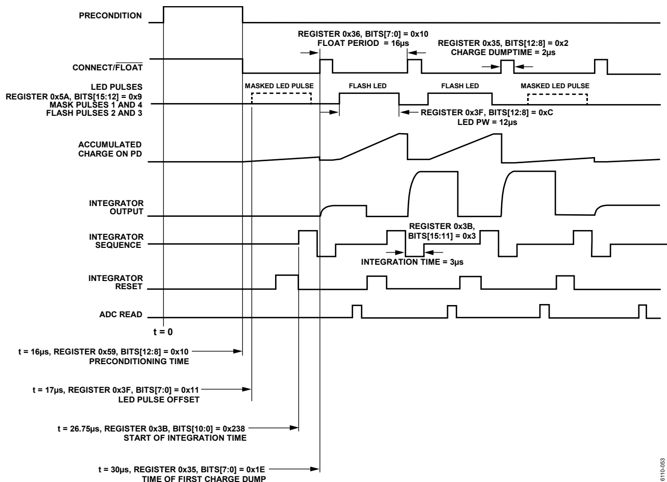
Figure 55. Example Timing Diagram of Four Pulse Float LED Mode Sequence
