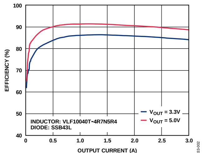
Figure 2. ADP2303 Efficiency vs. Output Current at V_{IN} = 12\text{ V}
