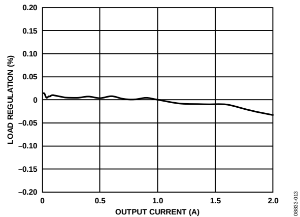
Figure 13. ADP2302 Load Regulation, V_{OUT} = 3.3\text{ V} , V_{IN} = 12\text{ V}
