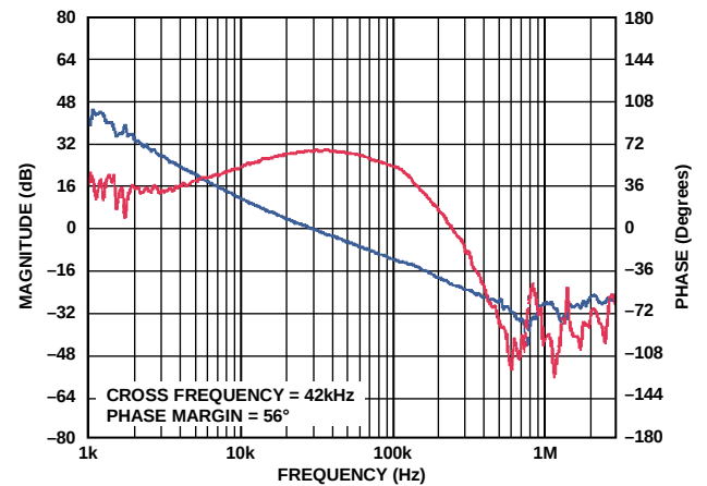
Figure 39. ADP2302 Bode Plot, V_{OUT} = 3.3\text{ V} , V_{IN} = 12\text{ V} , L = 6.8\text{ }\mu\text{H} , C_{OUT} = 2 \times 22\text{ }\mu\text{F}
