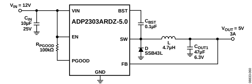
Figure 62. ADP2303 Typical Application, V_{IN} = 12\text{ V} , V_{OUT} = 5\text{ V} , 3\text{ A}
