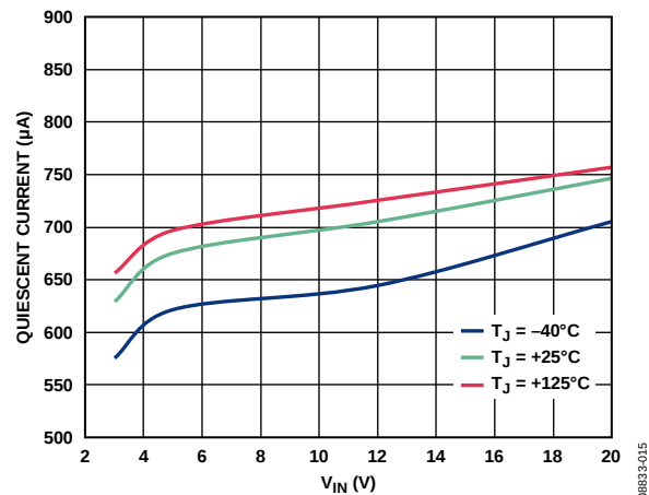
Figure 15. Quiescent Current vs. V_{IN}
