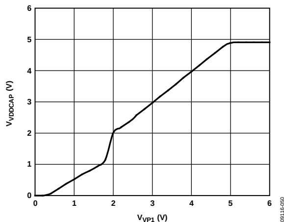
Figure 4. V_{VDDCAP} vs. V_{VP1}
