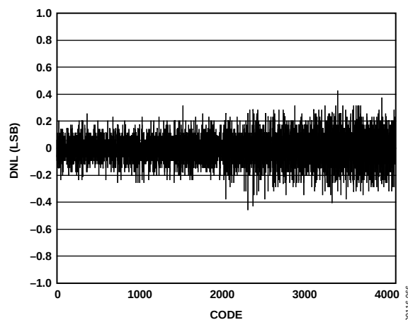
Figure 13. DNL for ADC
