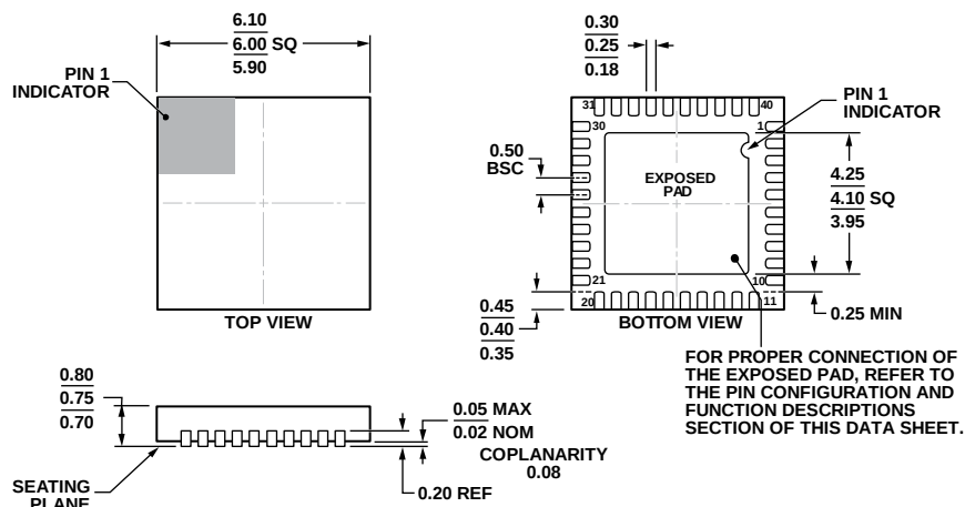
COMPLIANT TO JEDEC STANDARDS MO-220-WJJD. Figure 17. 40-Lead Lead Frame Chip Scale Package [LFCSP_WQ] 6 mm × 6 mm Body, Very Thin Quad (CP-40-9) Dimensions shown in millimeters
