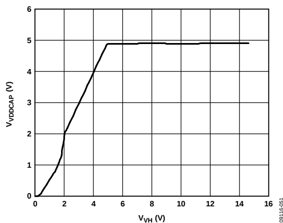
Figure 5. V_{VDDCAP} vs. V_{VH}
