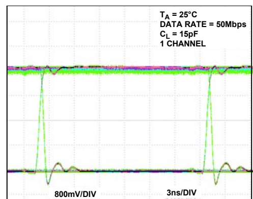
Figure 28. Eye Diagram at A Output (5 V \rightarrow 3.3 V Level Translation, 50 Mbps)
