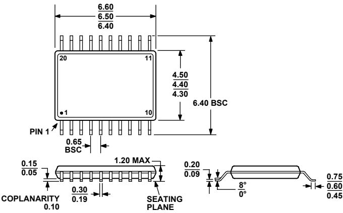
Figure 42. 20-Lead Thin Shrink Small Outline Package [TSSOP] (RU-20)
