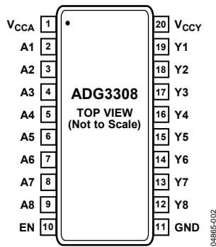
Figure 2. 20-Lead TSSOP
