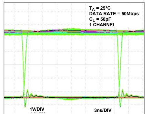
Figure 27. Eye Diagram at Y Output (3.3 V \rightarrow 5 V Level Translation, 50 Mbps)
