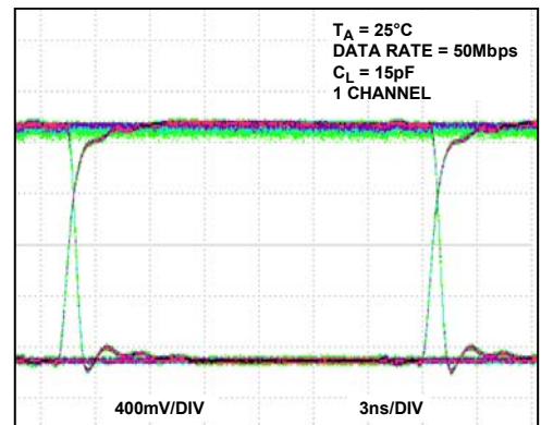
Figure 26. Eye Diagram at A Output (3.3 V \rightarrow 1.8 V Level Translation, 50 Mbps)
