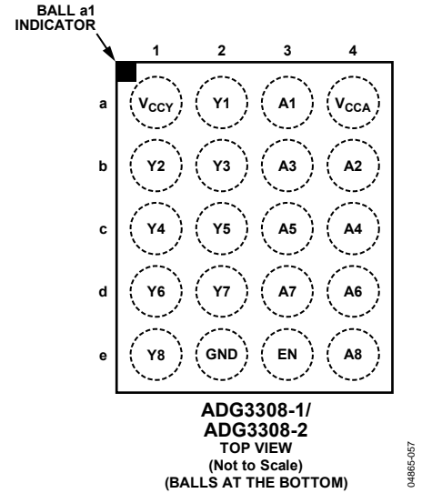
Figure 4. 20-Ball WLCSP
