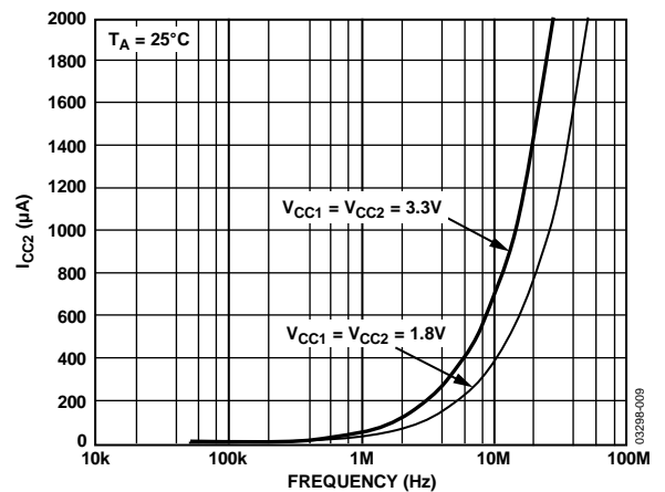
Figure 10. I_{CC2} vs. Frequency
