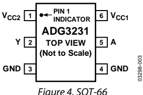
Figure 4. SOT-66
