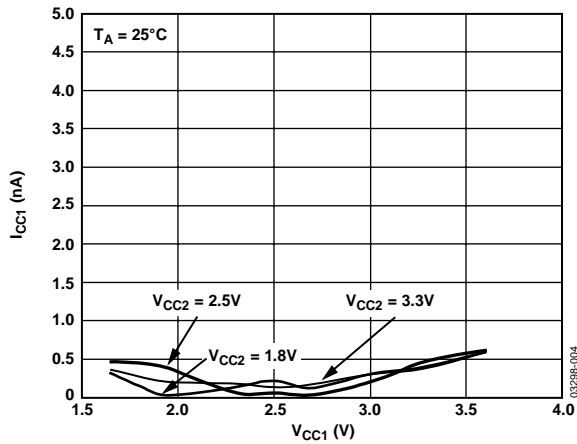
Figure 5. I_{CC1} vs. V_{CC1}
