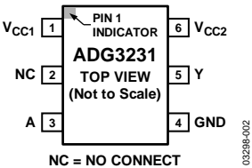
Figure 3. SOT-23
