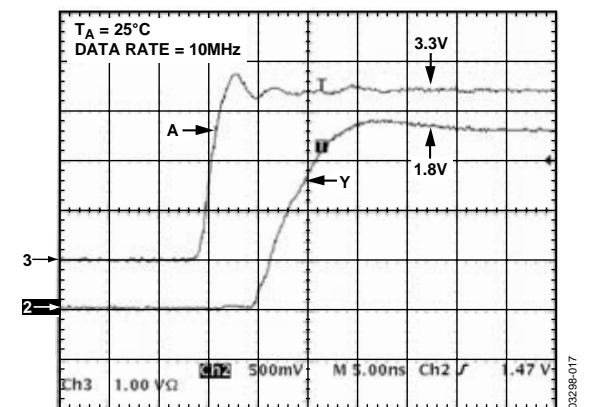
Figure 16. Input/Output V_{CC1} = 3.3\text{ V} , V_{CC2} = 1.8\text{ V}
