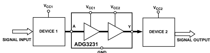
Figure 19. Typical Application of the ADG3231 Level Translator
