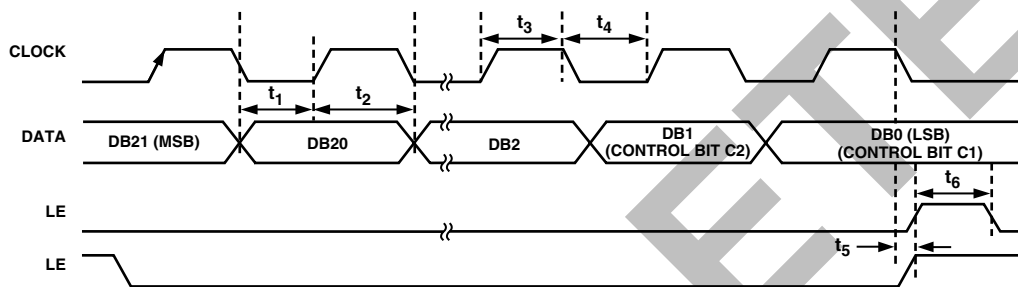
Figure 1. Timing Diagram
