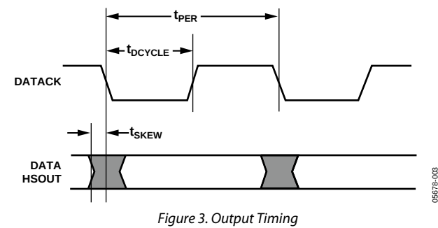
Figure 3. Output Timing
