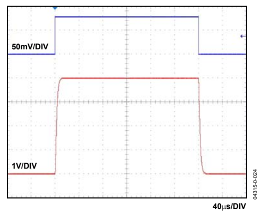
Figure 8. Rise/Fall Time
