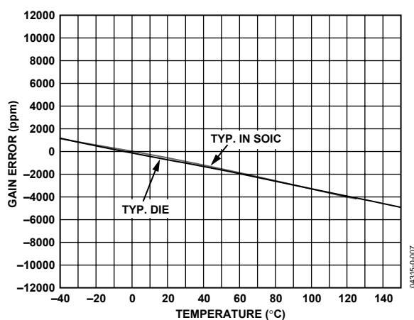
Figure 6. Gain Drift
