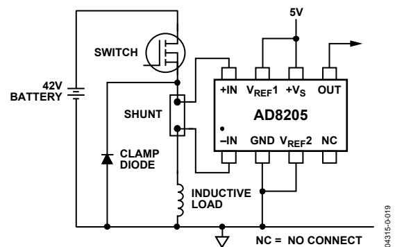
Figure 20. High-Side Switch
