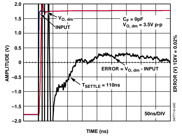
Figure 40. Settling Time (0.02%)
