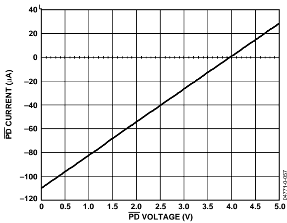
Figure 56. \overline{PD} Current vs. \overline{PD} Voltage
