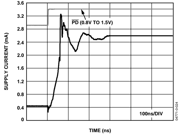
Figure 59. Power-Down Turn-On Time
