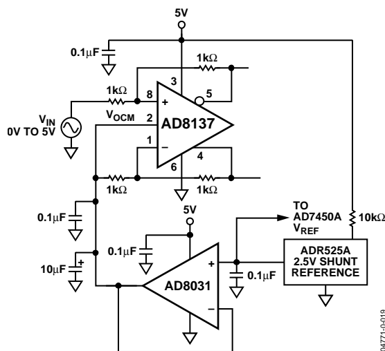
Figure 65. Low-Z Bias Source
