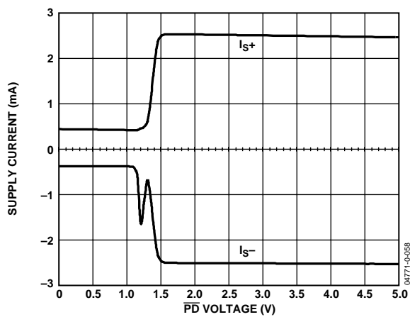
Figure 57. Supply Current vs. \overline{PD} Voltage
