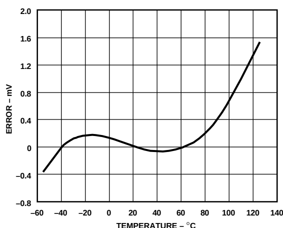
Figure 7. Typical AD780BN Temperature Drift
