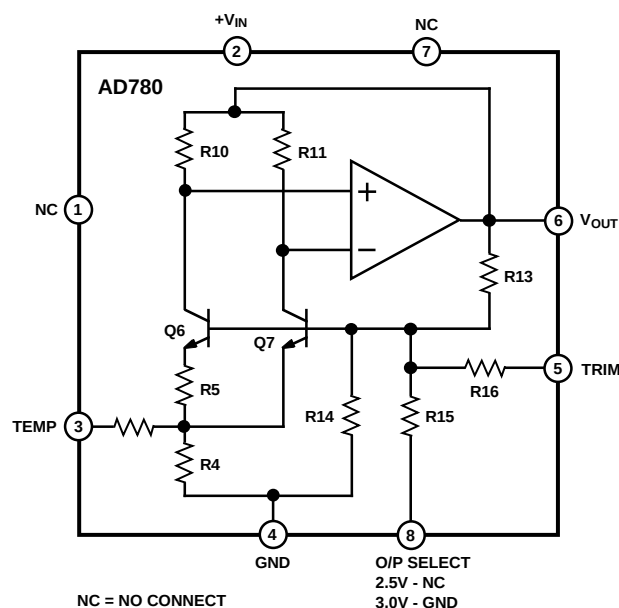
Figure 1. Schematic Diagram
