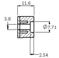
SECTION L-L SCALE 2:1
