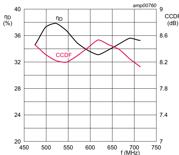
Fig 3. Drain efficiency and CCDF as function of frequency; typical values
