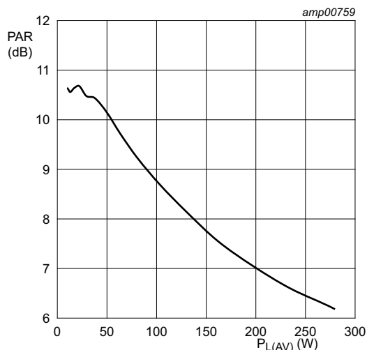
Fig 6. Peak-to-average power ratio as a function of average output power; typical values
