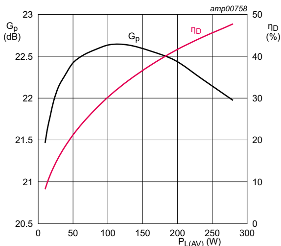
Fig 5. Power gain and drain efficiency as function of average output power; typical values
