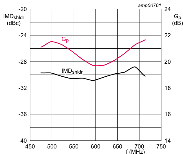
Fig 4. Intermodulation distortion shoulder and power gain as function of frequency; typical values
