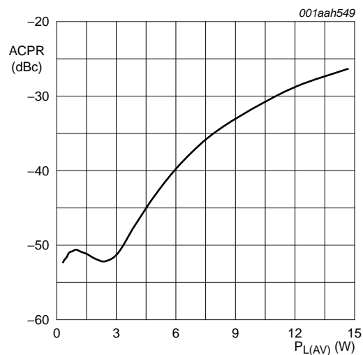
Fig 5. 2-carrier W-CDMA adjacent power channel ratio as function of average load power; typical values
