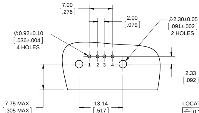
RECOMMENDED PCB LAYOUT COMPONENT SIDE OF BOARD
