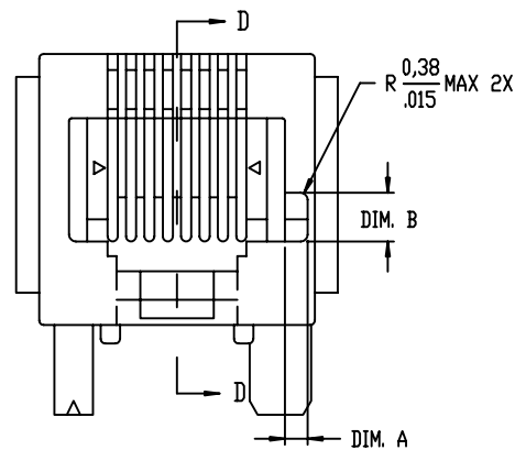
KEYED STYLE
