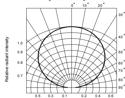
Fig.6 Radiation diagram
