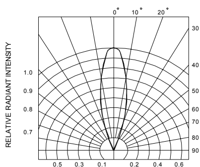
RADIATION DIAGRAM
