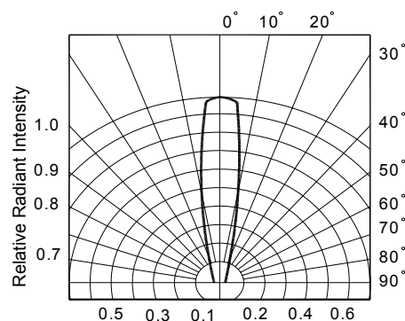
FIG.6 Radiant Diagram
