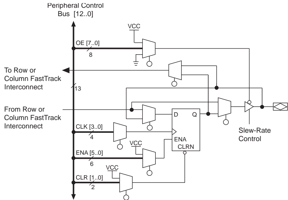
Figure 10. MAX 9000 IOC
