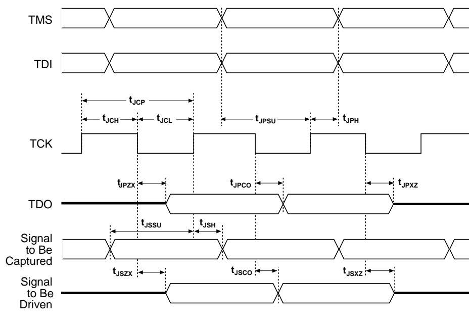
Figure 11. MAX 9000 JTAG Waveforms
