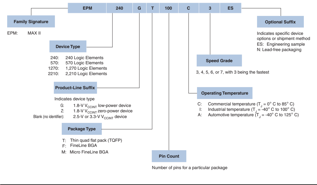
Figure 6–1. MAX II Device Packaging Ordering Information
