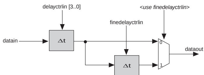
Figure 8-22. Delay Chain
