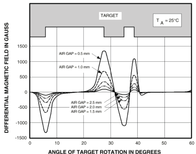
Figure 4. Effect of varying air gaps on differential circuits.
