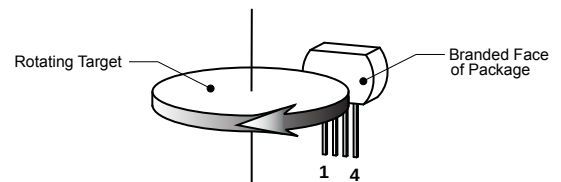
Figure 6. This left-to-right (pin 1 to pin 4) direction of target rotation results in a high output signal when a tooth of the target gear is nearest the branded face of the package. A right-to-left (pin 4 to pin 1) rotation inverts the output signal polarity.
