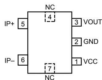
Pinout Diagram
