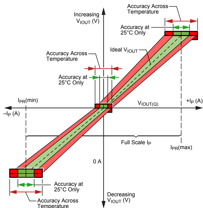
Figure 11: Output Voltage versus Sensed Current
