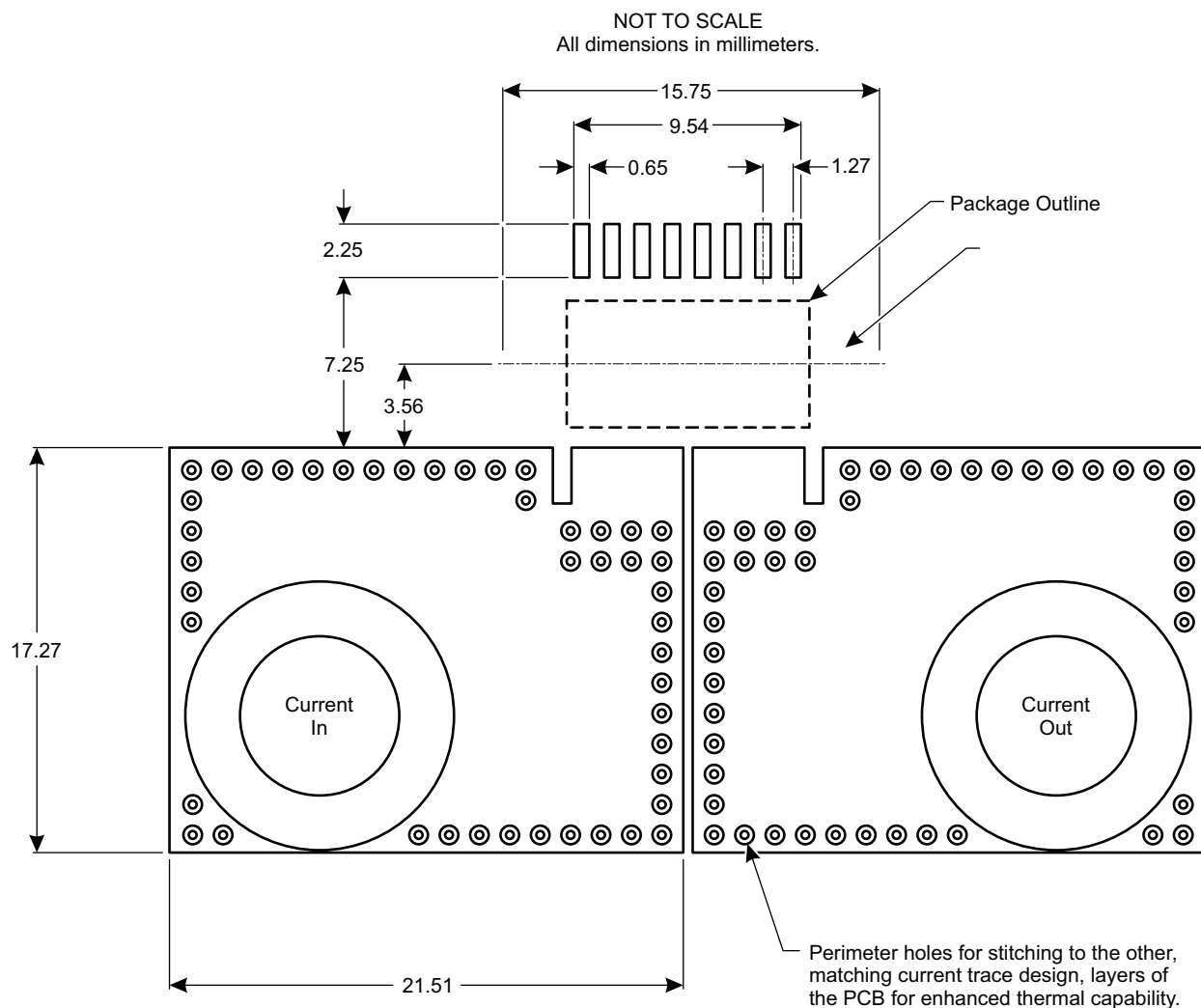
Figure 16: High Isolation PCB Layout
