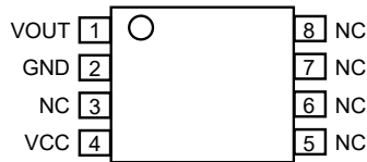
Figure 4: Pinout Diagram
