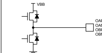
Figure 18i. Phase Outputs
