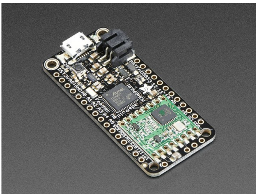
Adafruit Feather M0 RFM69HCW Packet Radio - 868 or 915 MHz
