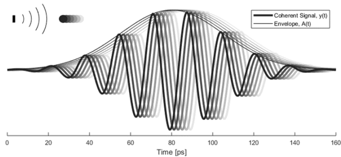
Fig. 2.5: Illustration of envelope and phase change of a received pulse for a reflection from a moving object, what is returned from the IQ Service is in cartesian form.
