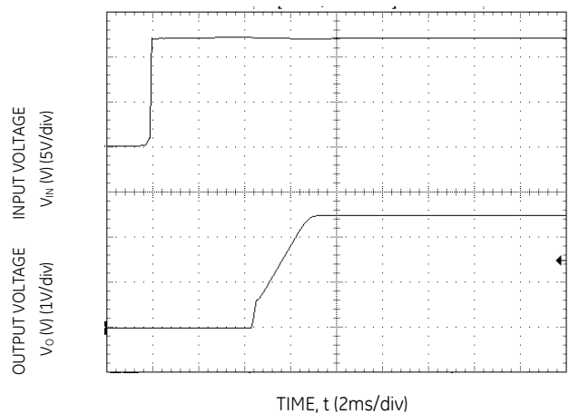
Figure 24. Typical Start-up Using Input Voltage ( V_{IN}=12\text{V} , I_o=I_{o,max} ).
