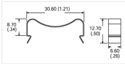
Standard Clip for heat sink attachment
