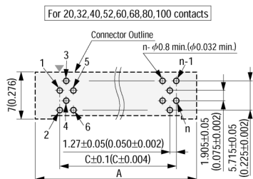
Printed Circuit Board Layout (Component Side View)
